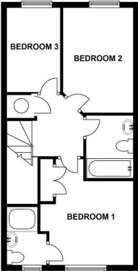
FIRST FLOOR APPROX. 39.8 SQ. METRES (428.4 SQ. FEET)
